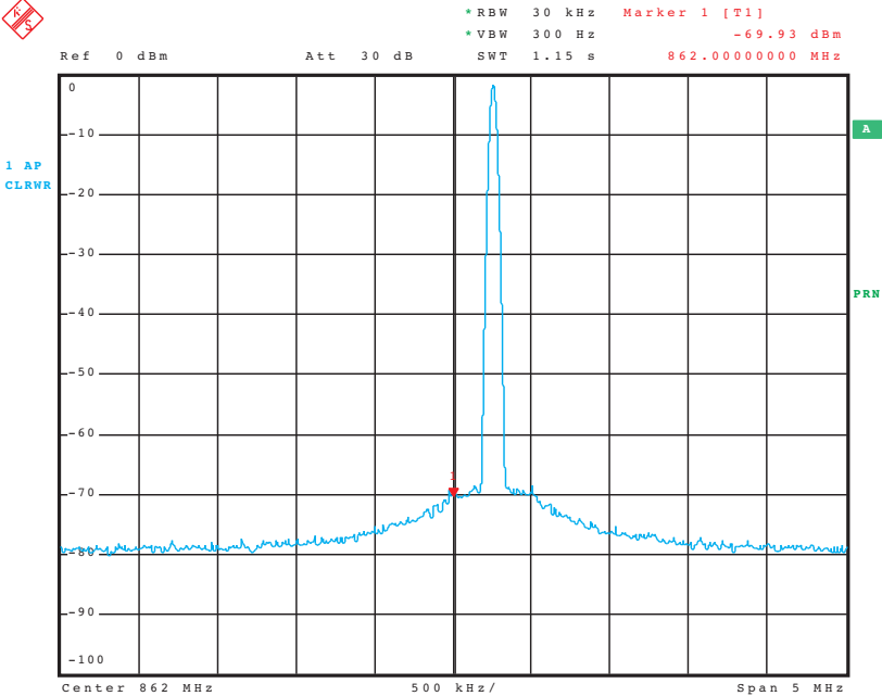
Fig. 4-39 Mixture products due to overdriving of A/D converter converter when using digital IF filters or FFT filters (a); displayed spectrum in case of correct driving (b)
