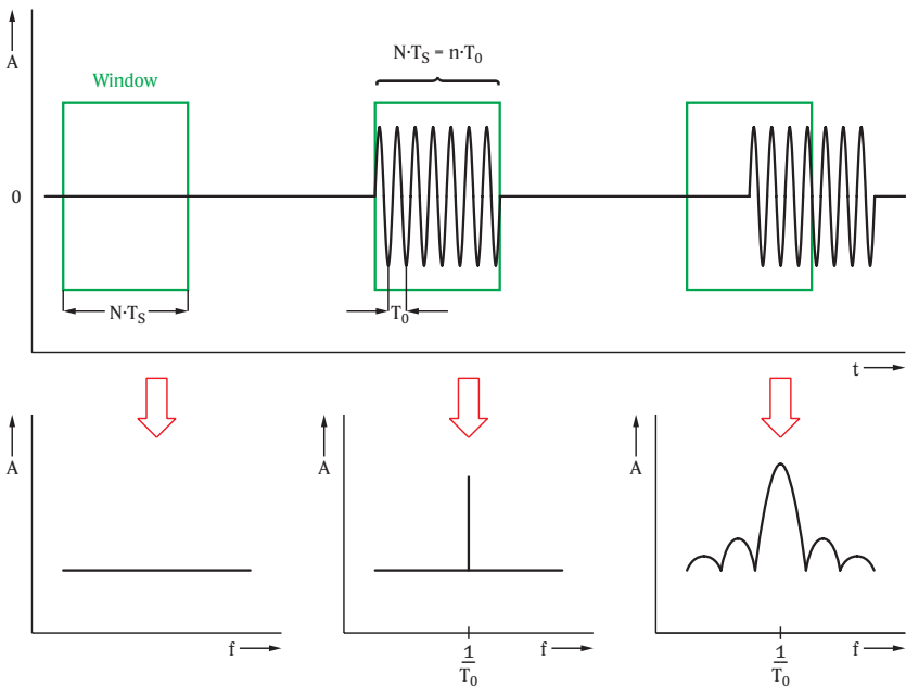
Fig. 3-7 FFT of pulsed signals. The result depends on the time of the measurement
