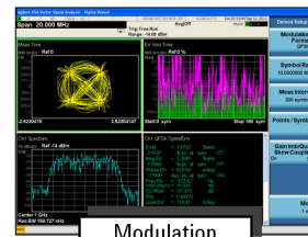
Modulation
