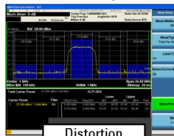
Distortion
