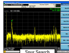
Spur Search
