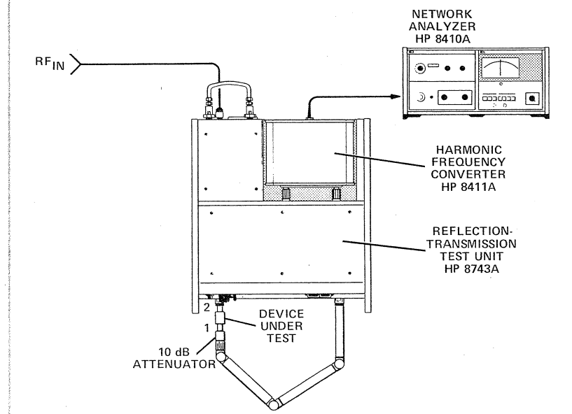
b) Setup for Measuring S_{22} and S_{12}
