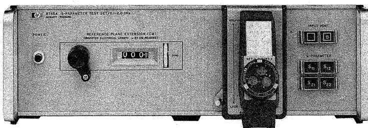
HP 8745A with the 11600B Transistor Fixture attached
