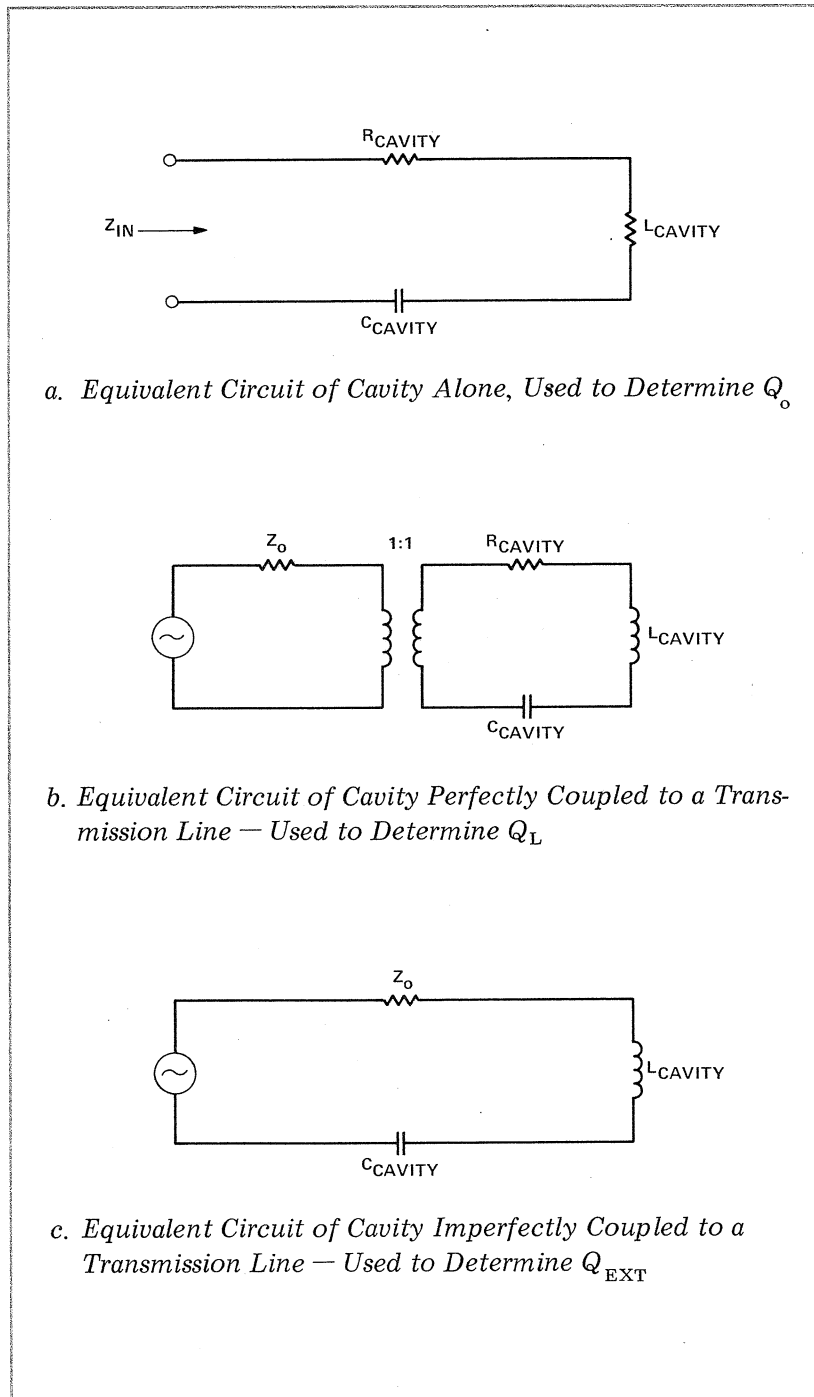
Figure 8-12. Cavity Equivalent Circuits
