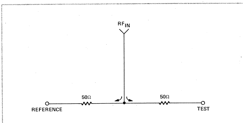
Figure 2-11. Power Splitter
