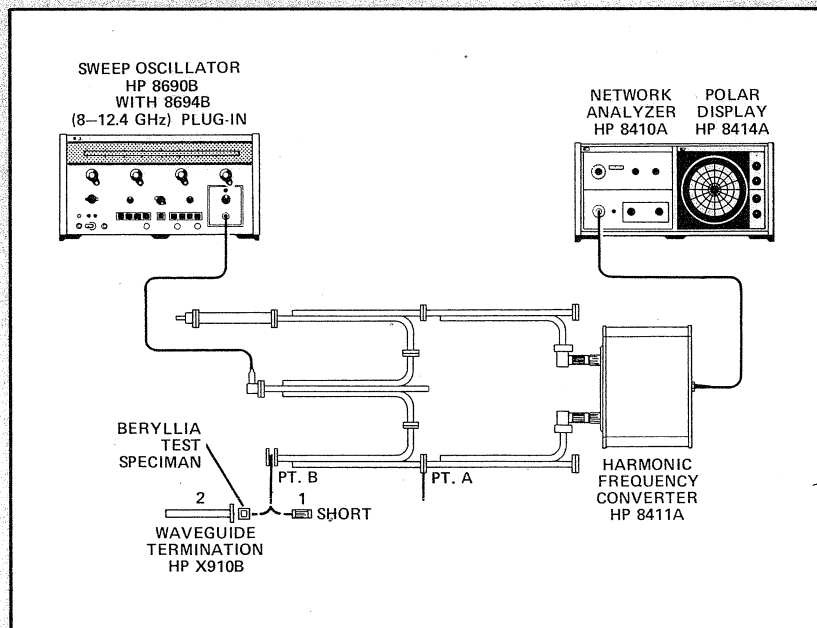
Figure 7-6. Equipment Setup
