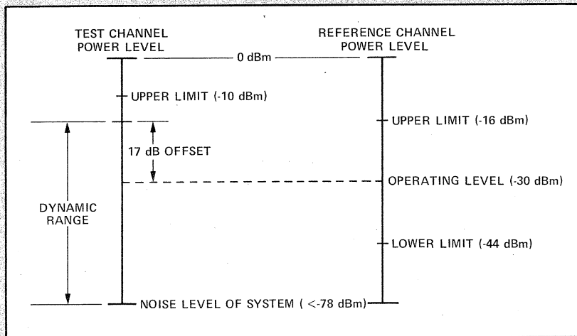
Figure 3-5. Power Levels for Attenuation Measurements
