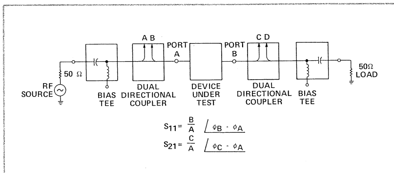
Figure 4-2. Setup for Measuring S_{11} and S_{21}
