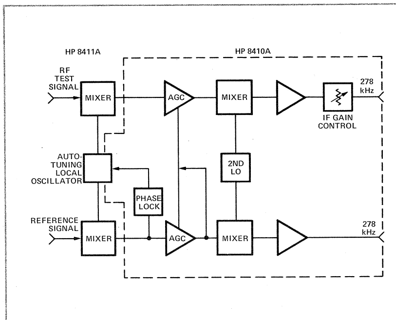
Figure 2-4. Simplified Block Diagram of the Harmonic Frequency Converter (8411A) & Network Analyzer (8410A)
