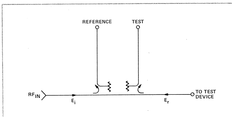
Figure 2-12. Dual Directional Coupler
