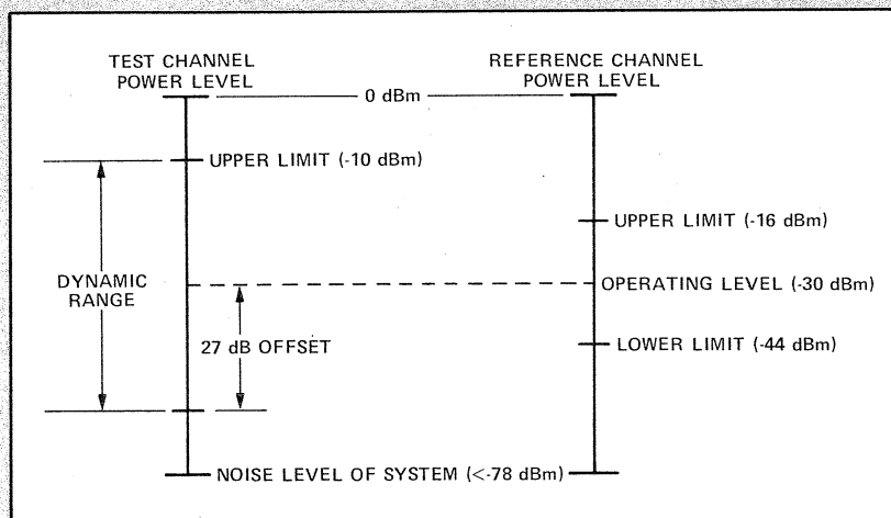
Figure 3-6. Power Levels for Gain Measurements
