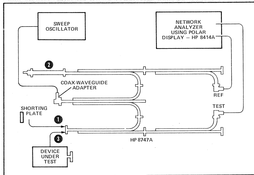
Figure 7-3. 8747A Reflection Test Setup
