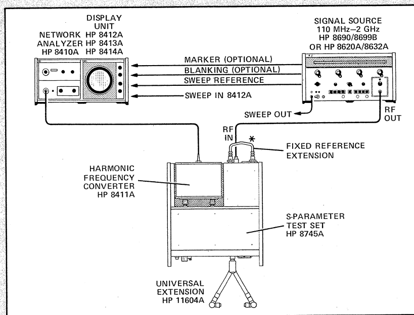
Figure 4-5. General Test Setup for Microwave Hardware Measurements Using the 8745A S-Parameter Test Set
