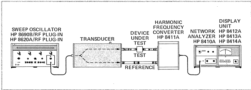
Transducer used in a Transmission Measurement
