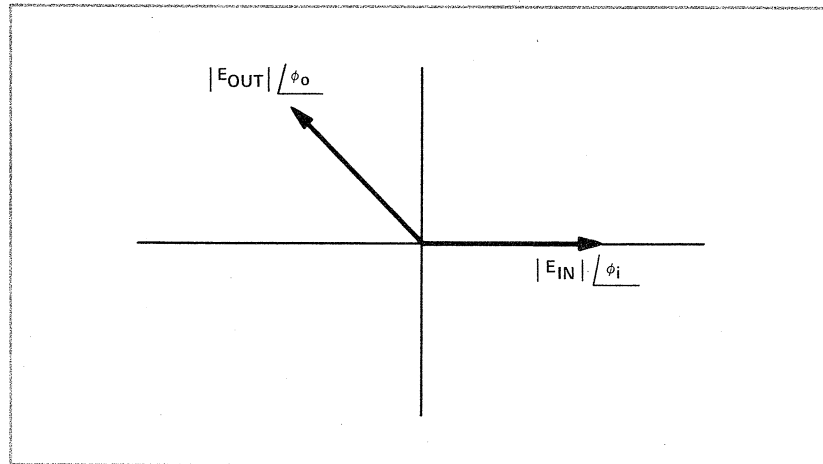
Figure 1-5. Typical Magnitude and Phase Relationships In a Transmission Test
