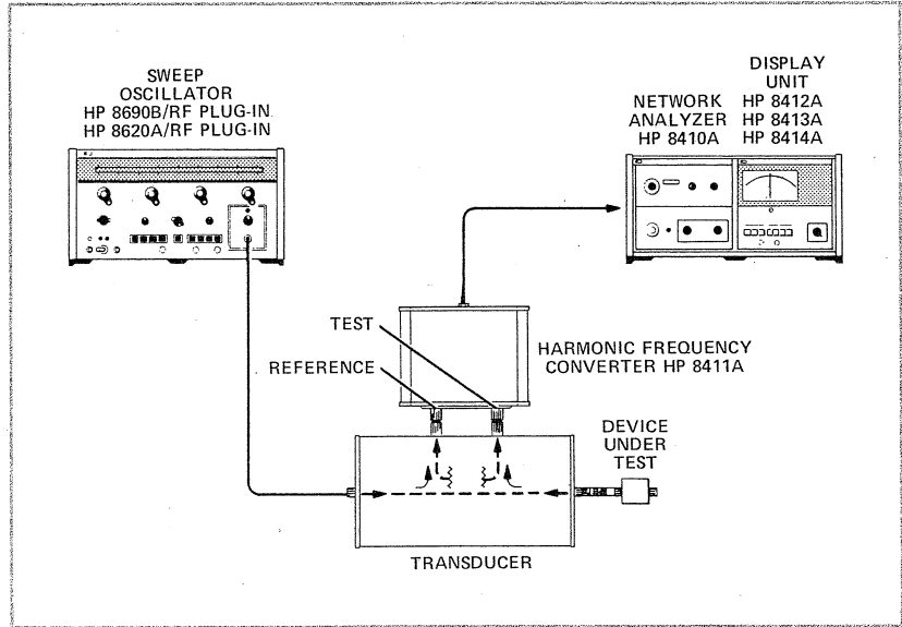
Figure 2-2. Reflection Measurement
