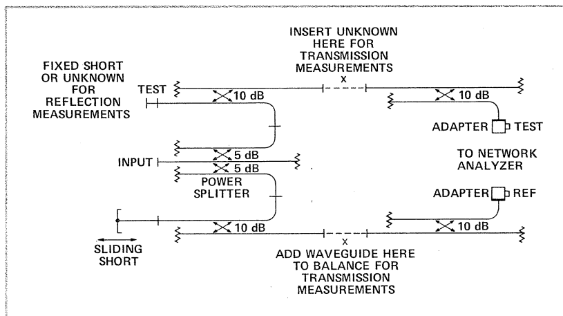
Figure 7-2. HP 8747A Schematic
