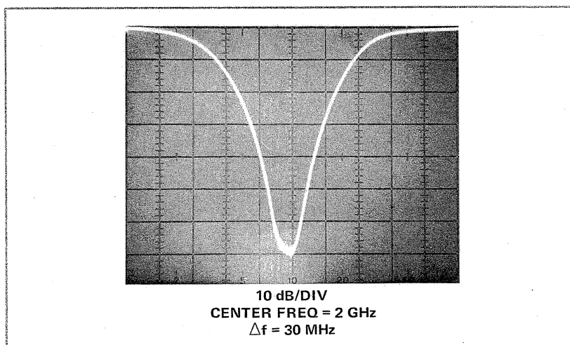
Figure 2-6. Test Results using the 8412A in a Transmission Measurement of an HP 8739A Notch Filter
