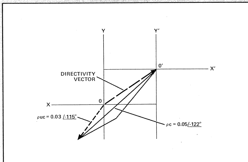
Figure 5-11. Vector Relationships
