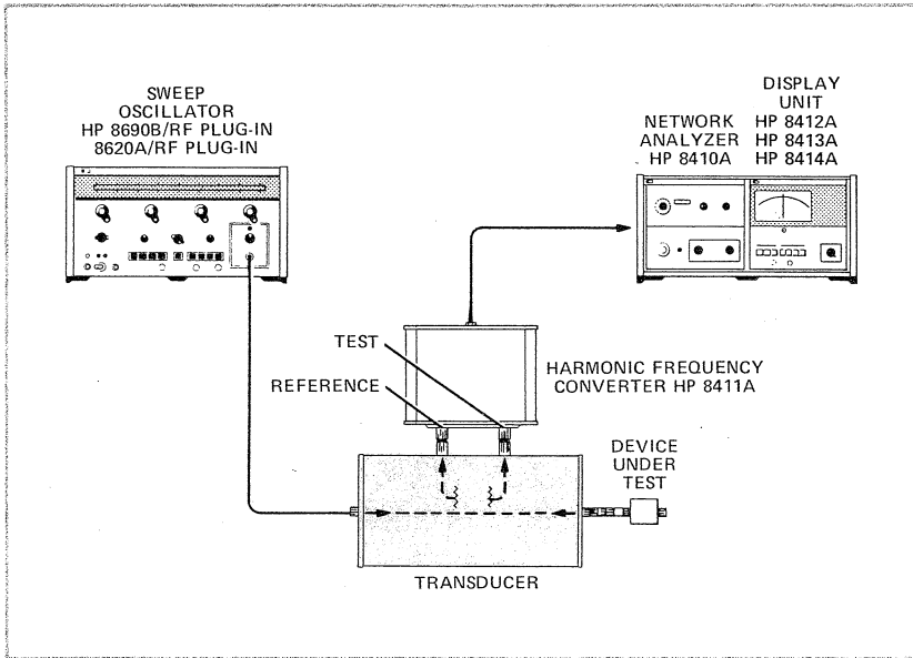
Transducer used in a Reflection Measurement
