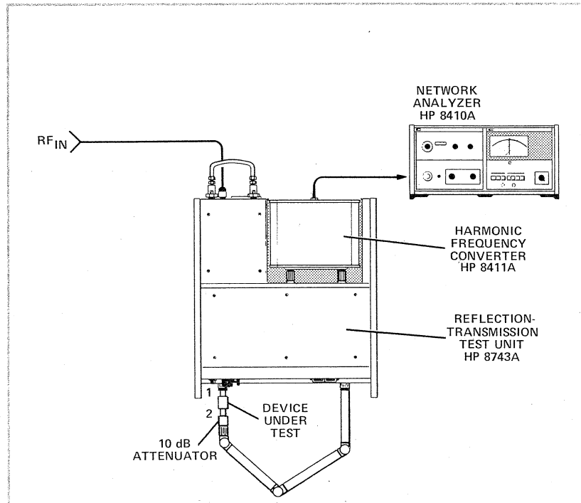
a) Setup for Measuring S_{11} and S_{21}
