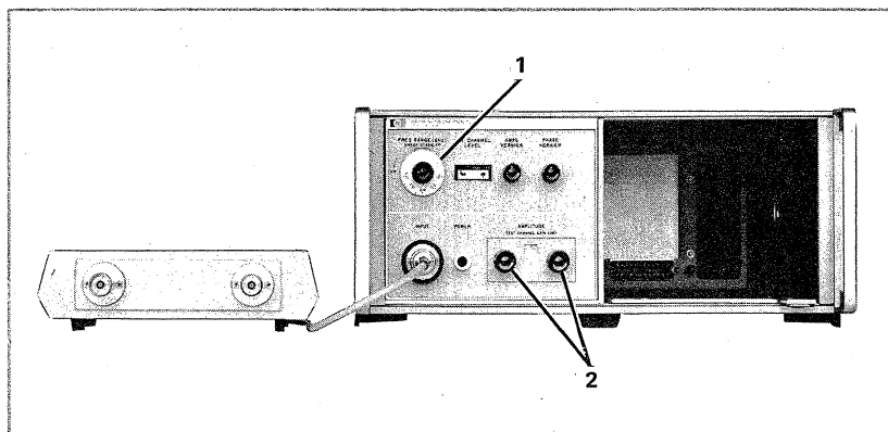
Figure 2-3. The Harmonic Frequency Converter and Network Analyzer Mainframe
