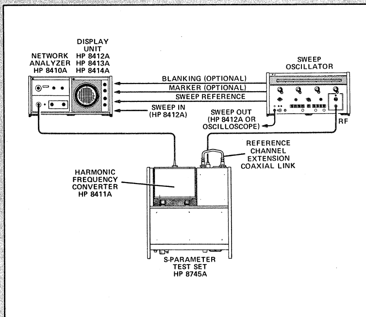
Figure 1. Cable Connections When Using the 8745A
