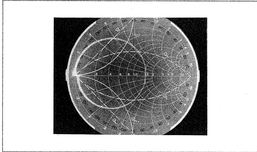
Figure 8-6. Cavity Resonance
