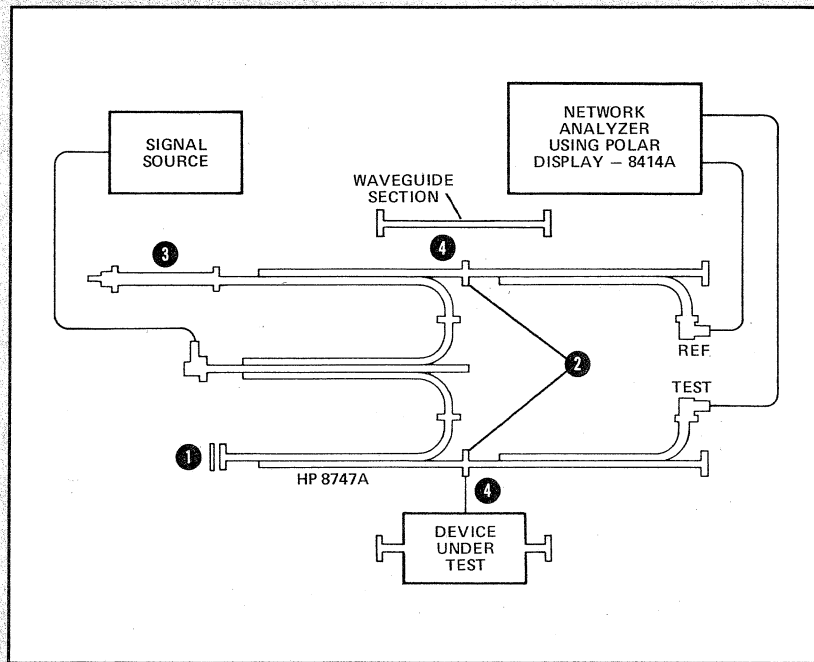
Figure 7-4. HP 8747A Transmission Test Setup
