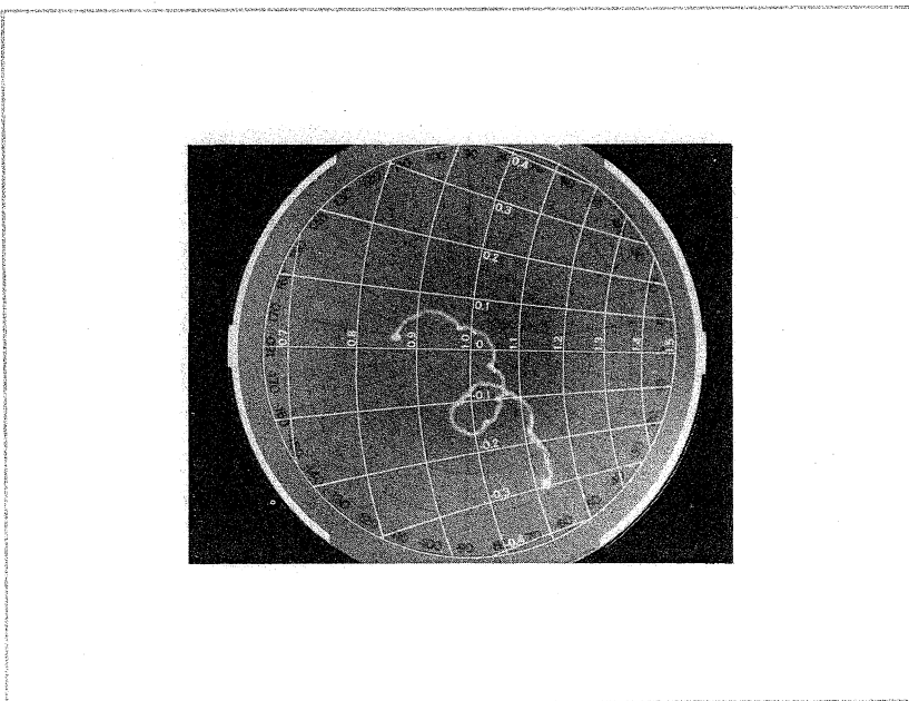
Figure 8-1. Antenna Impedance
