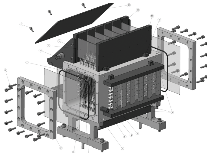
Figure 8. Beam Monitor mechanical drawing.
